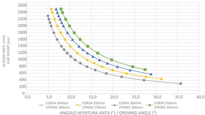
LIWIN L40 SLIM 350 - VASISTAS LIWIN L40 SLIM 350 - BOTTOM HANG OPENING ANGLE
