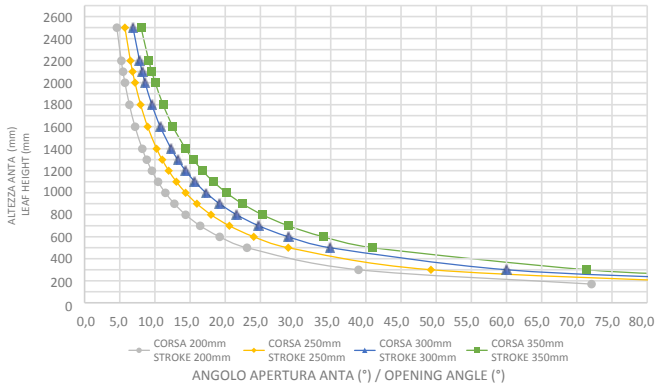
LIWIN L40 SLIM 350 - SPORGERE LIWIN L40 SLIM 350 - TOP HANG OPENING ANGLE
