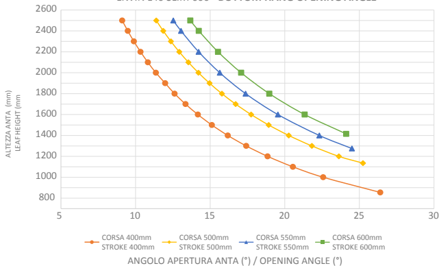
LIWIN L40 SLIM 600 - VASISTAS LIWIN L40 SLIM 600 - BOTTOM HANG OPENING ANGLE
